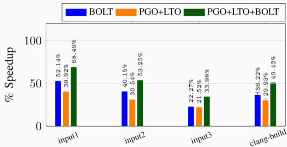
Cumulative speedup over bootstrapped build, Building Clang
