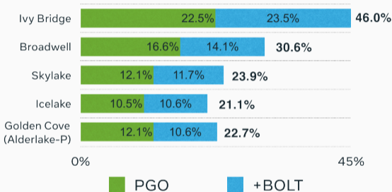
Cumulative speedup over bootstrapped build, Building Clang
